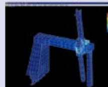
The machine structure has been optimized using FEM (Finite-Element Method) and modal analysis.
